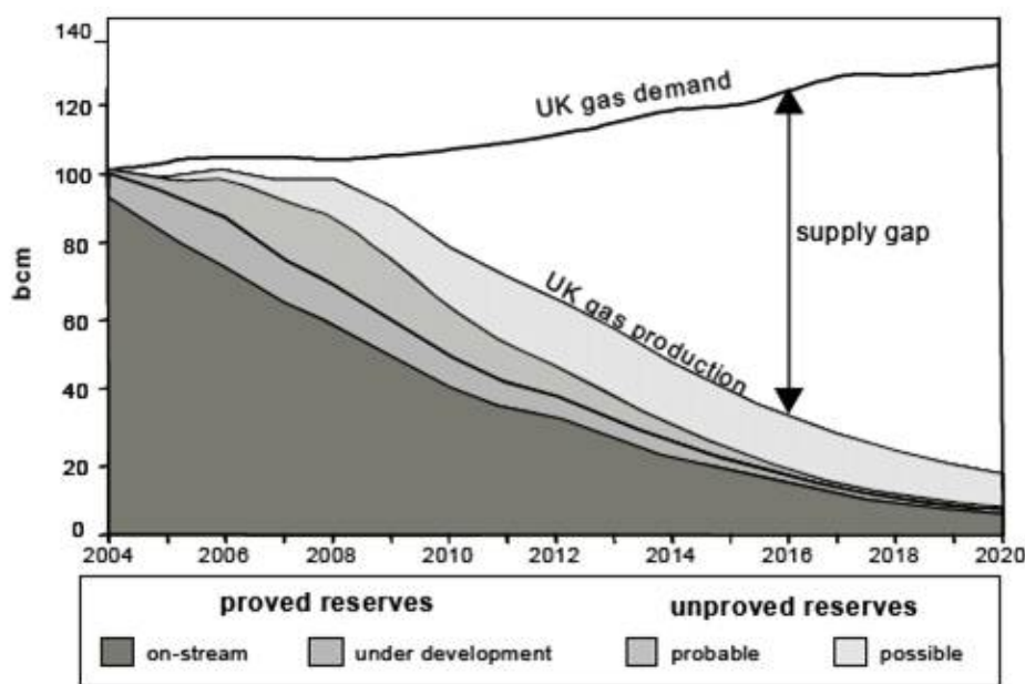
Figure 12: The forecasts for UK natural gas production to 2020, showing a precipitous decline over the next seven years. Source: Parliamentary Office of Science and Technology (2004)
